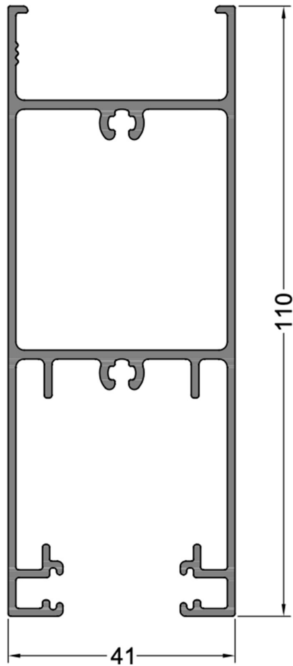
4260 1.537 Kg/m CORREDIZA HOJA UMBRAL DVH
